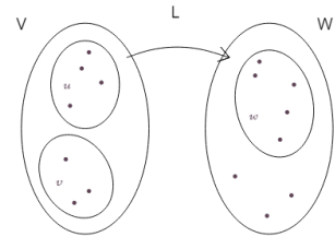
Figure 1: Representation of Thm 2.5 Note that the v_i are not necessarily uniquely determined!
