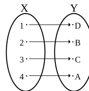
Figure 4: Bijective map.
