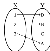
Figure 2: Injective (non surjective) map.
